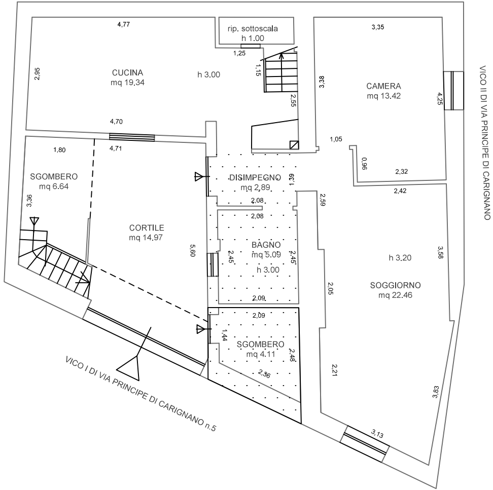
PIANO TERRA
